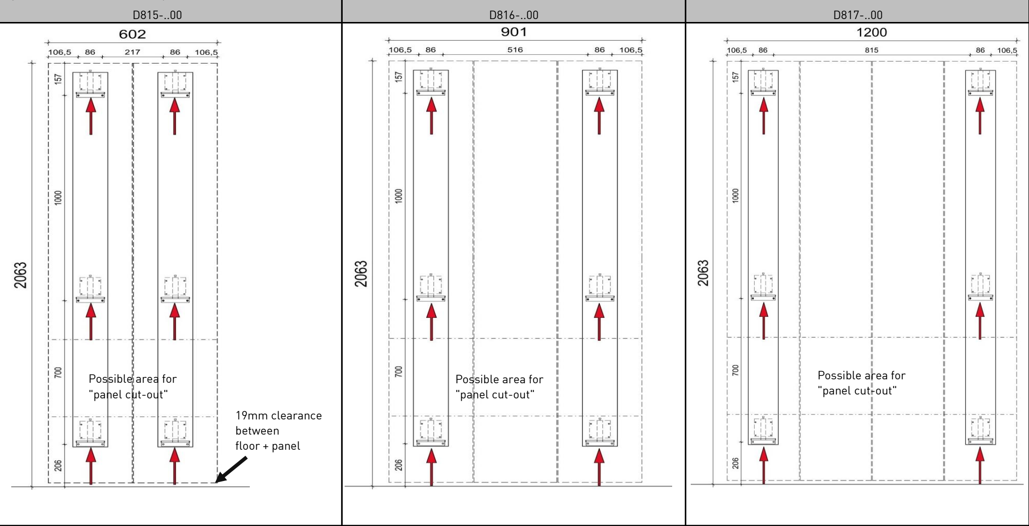
Fig. 4: Bore dimensions for suspension rails
