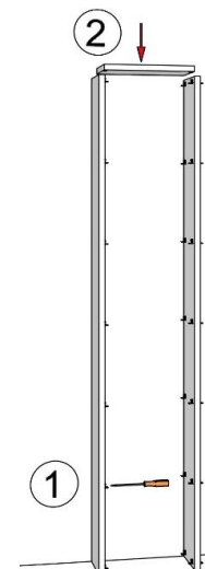
Fig. 3: Unit and shelf assembly
