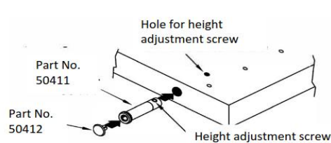
Fig. 2: Height adjuster assembly
