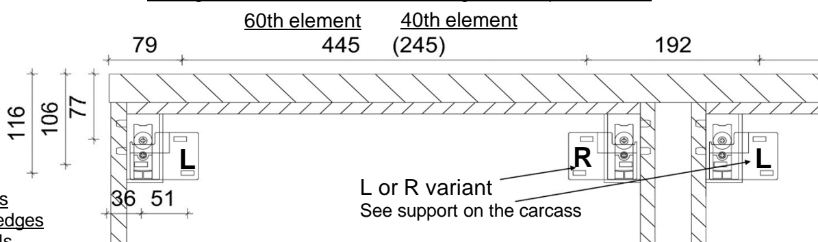
Drilling dimensions of carcass outer edges for suspension rails
