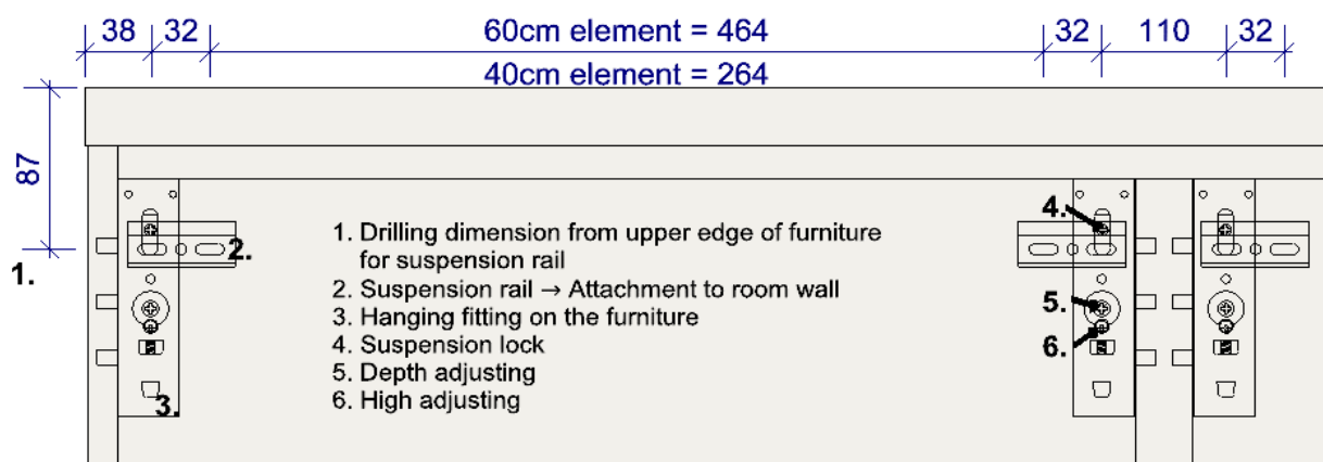
Figure 1: Drill dimensions (in mm) for suspension rail
