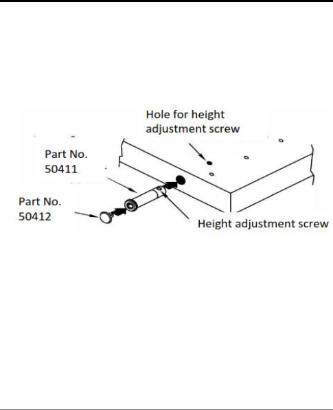
Fig. 2: Height adjuster assembly
