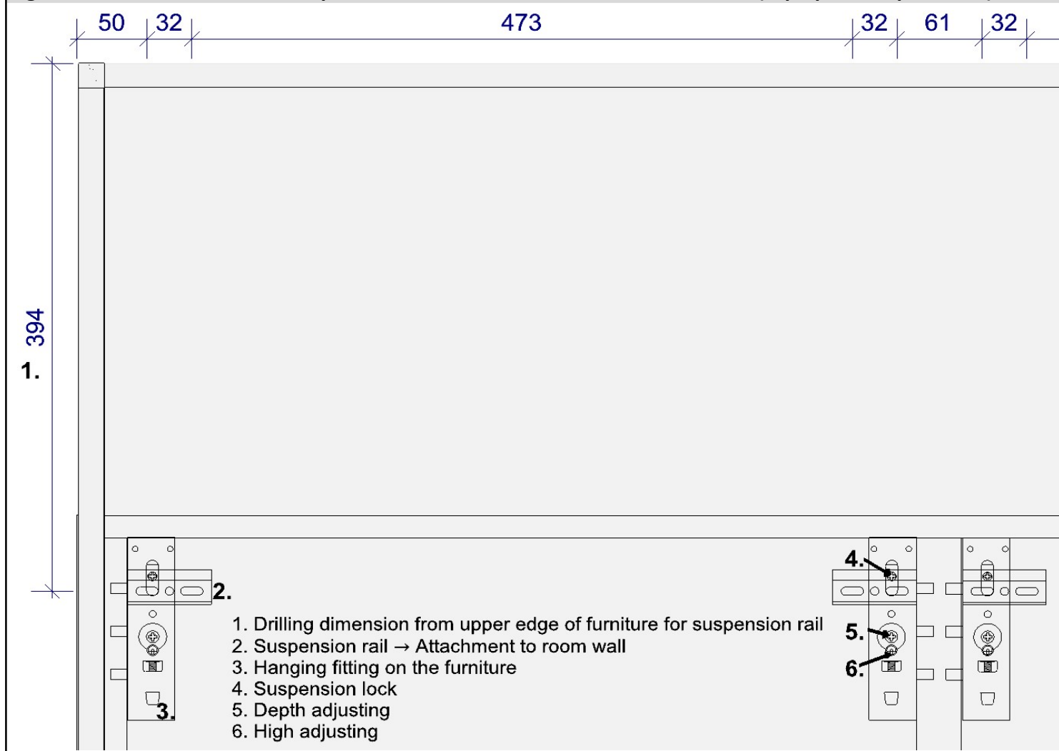
Figure 2: Drill dimensions for suspension elements W732, W733, W736, W737 (top open compartment)
