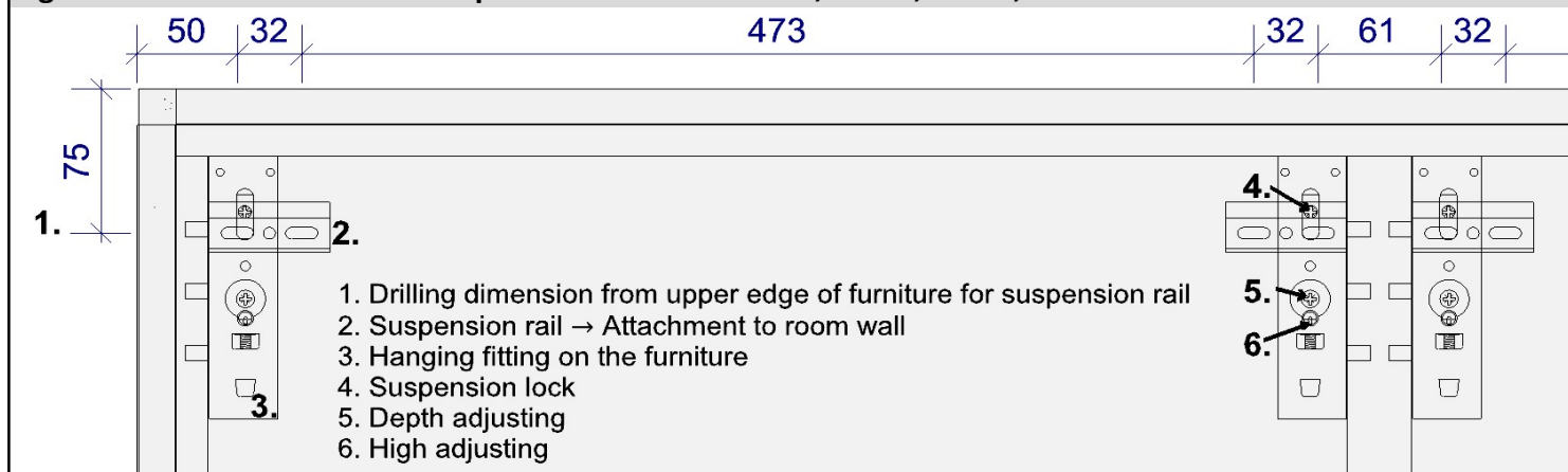
Figure 2: Drill dimensions for suspension elements W732, W733, W736, W737 (top open compartment)
