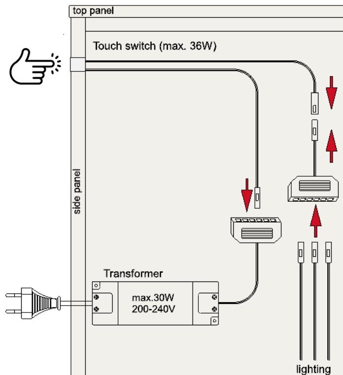
Figure 3: Wiring diagramm
