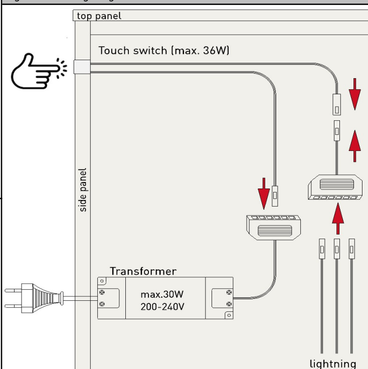
Figure 3: Wiring diagramm
