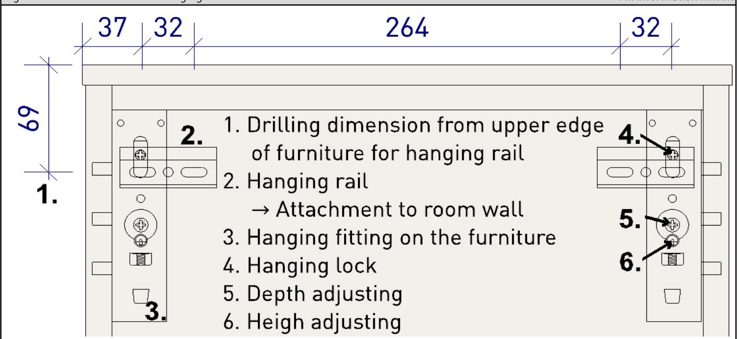
Figure 1: Drill dimensions for hanging rail
