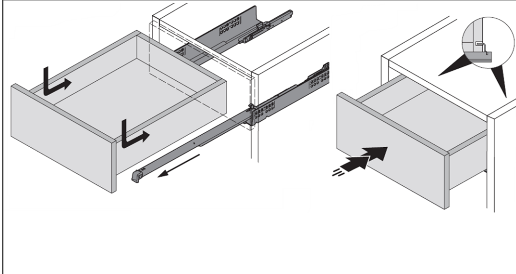
Figure 2: assembly drawer
