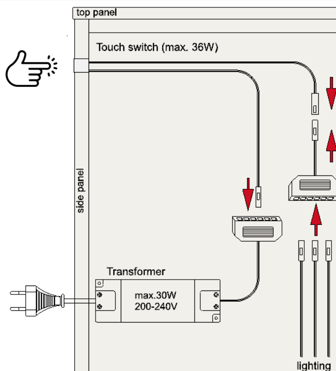
Figure 3: Wiring diagramm
