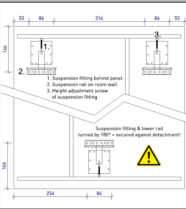
Figure 1: position suspension rails
