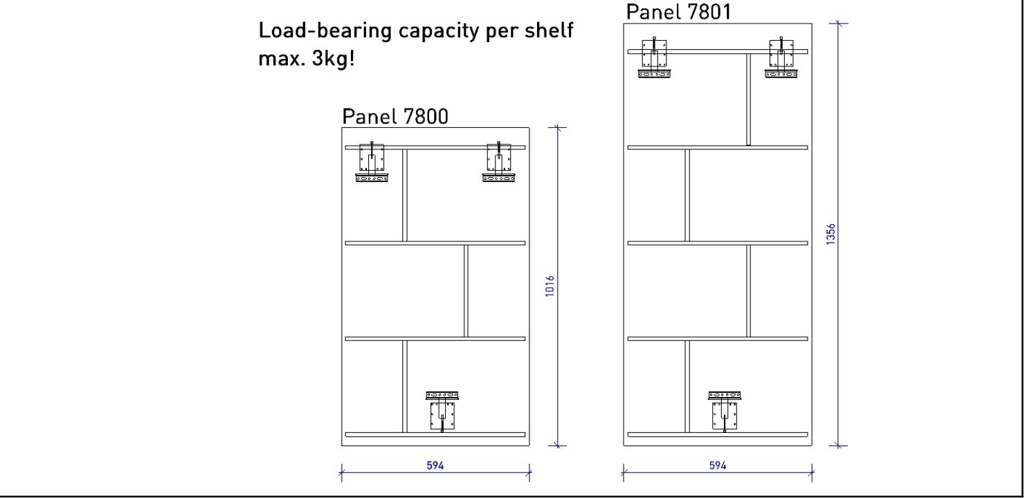
Figure 2: Panel types and fitting position
