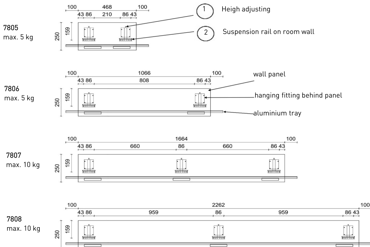
Figure 1: Drilling dimensions for suspension rails of wallpanel
