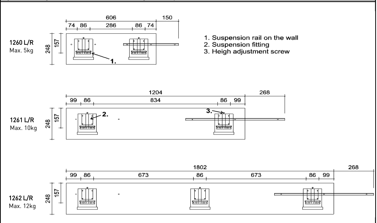
Figure 1: Drilling dimensions of wall shelf outer edges for suspension rails
