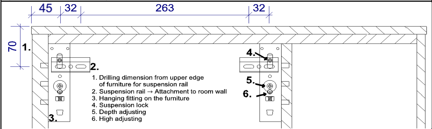
Figure 2: Drill dimensions for suspension rail (modell 5247)
