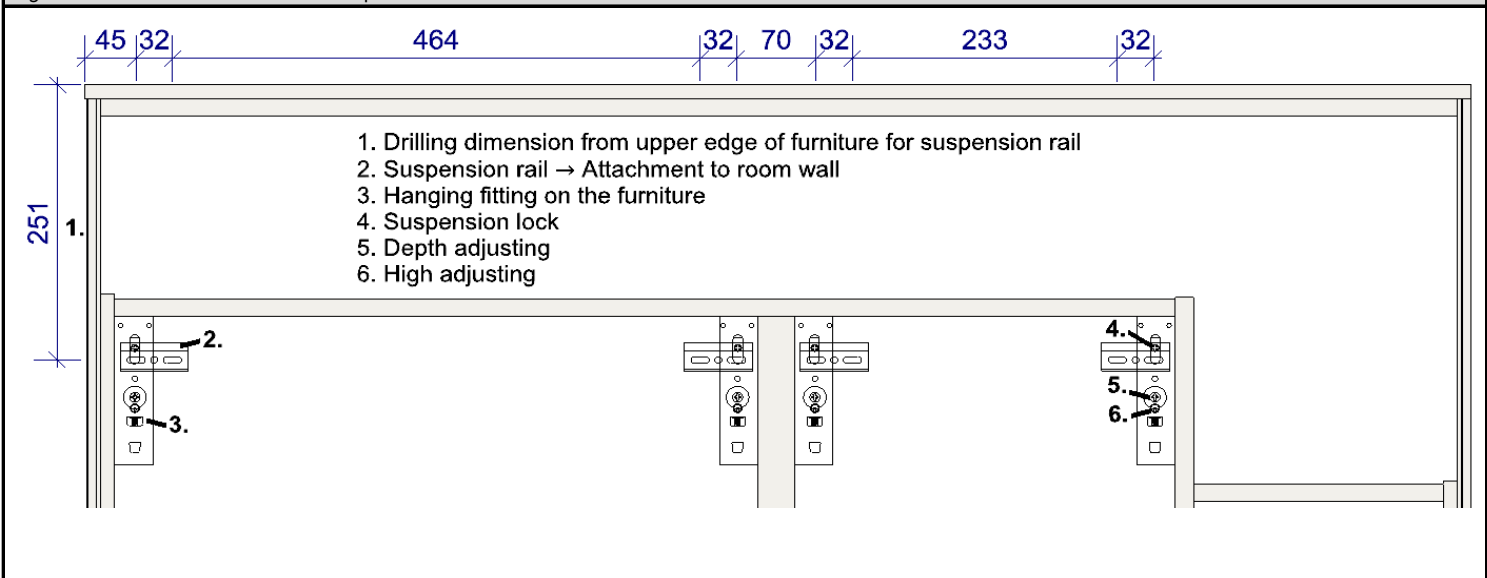
Figure 3: Drill dimensions for suspension rail (modell 5248)
