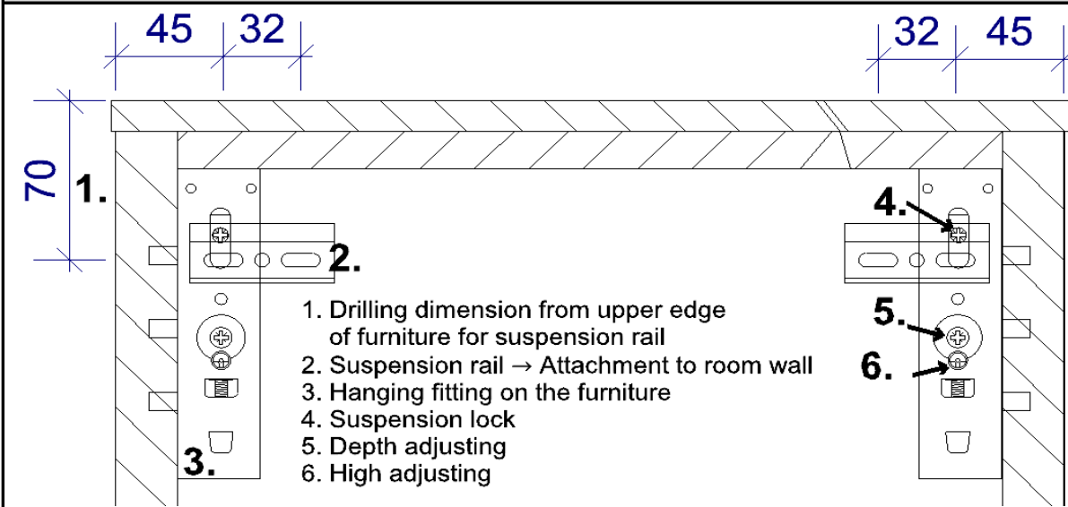
Figure 1: Drill dimensions for suspension rail (modell 5245 &amp; 5246)
