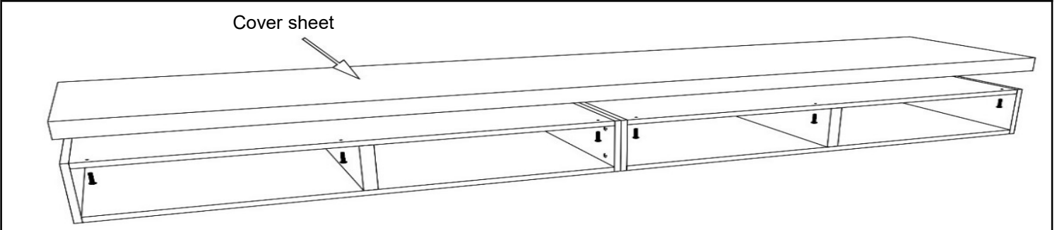
Figure 4: Fastening the cover sheet
