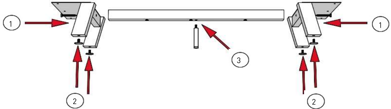
Fig. 2: wooden underframe
