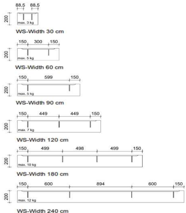
Figure 2: Overview of Wallboard sizes and load capacity
