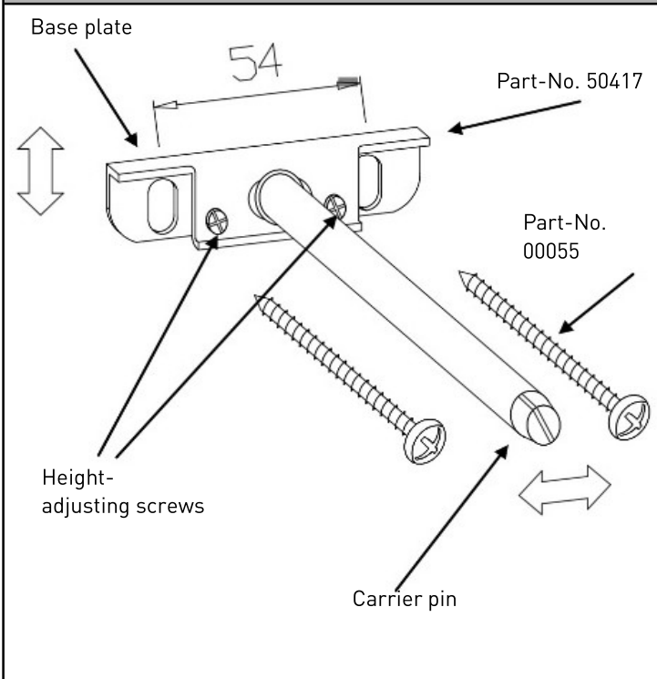
Figure 1: Detail of shelf support
