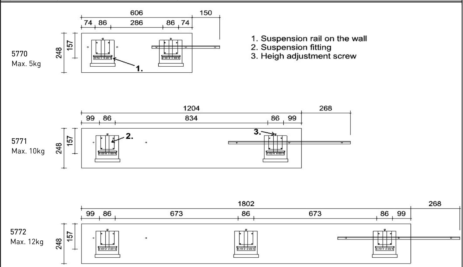
Figure 1: Drilling dimensions of wall shelf outer edges for suspension rails
