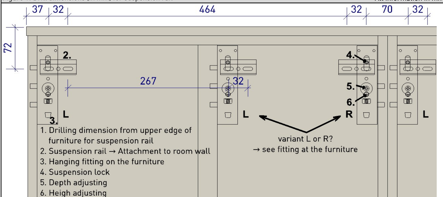
Figure 1: Drill dimensions (in mm) for suspension rail
